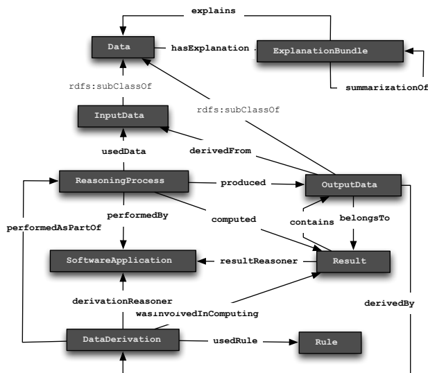
Fig. 1: The core classes and properties of Ratio4TA .
